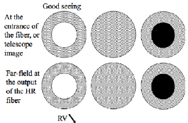
Fig. 4. When the seeing is good, the telescope image is less wide. With the double scrambler in HR mode, near field becomes far-field and is projected on the collimator at the entrance of the spectrograph. The pattern is comparable to that observed in HE when vignetting telescope (Fig. 2)
