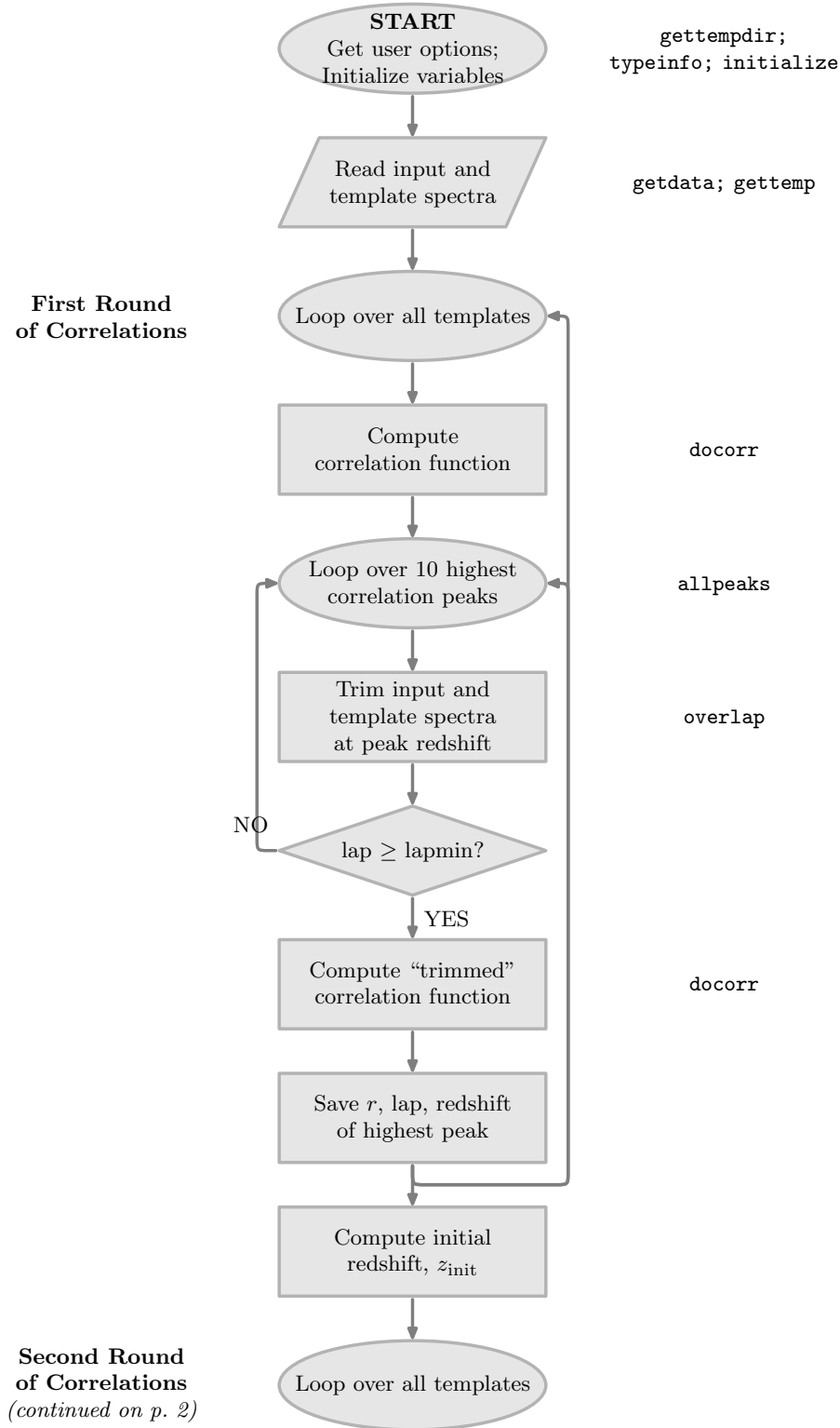
Figure 1 SNID v5.0 Flowchart
