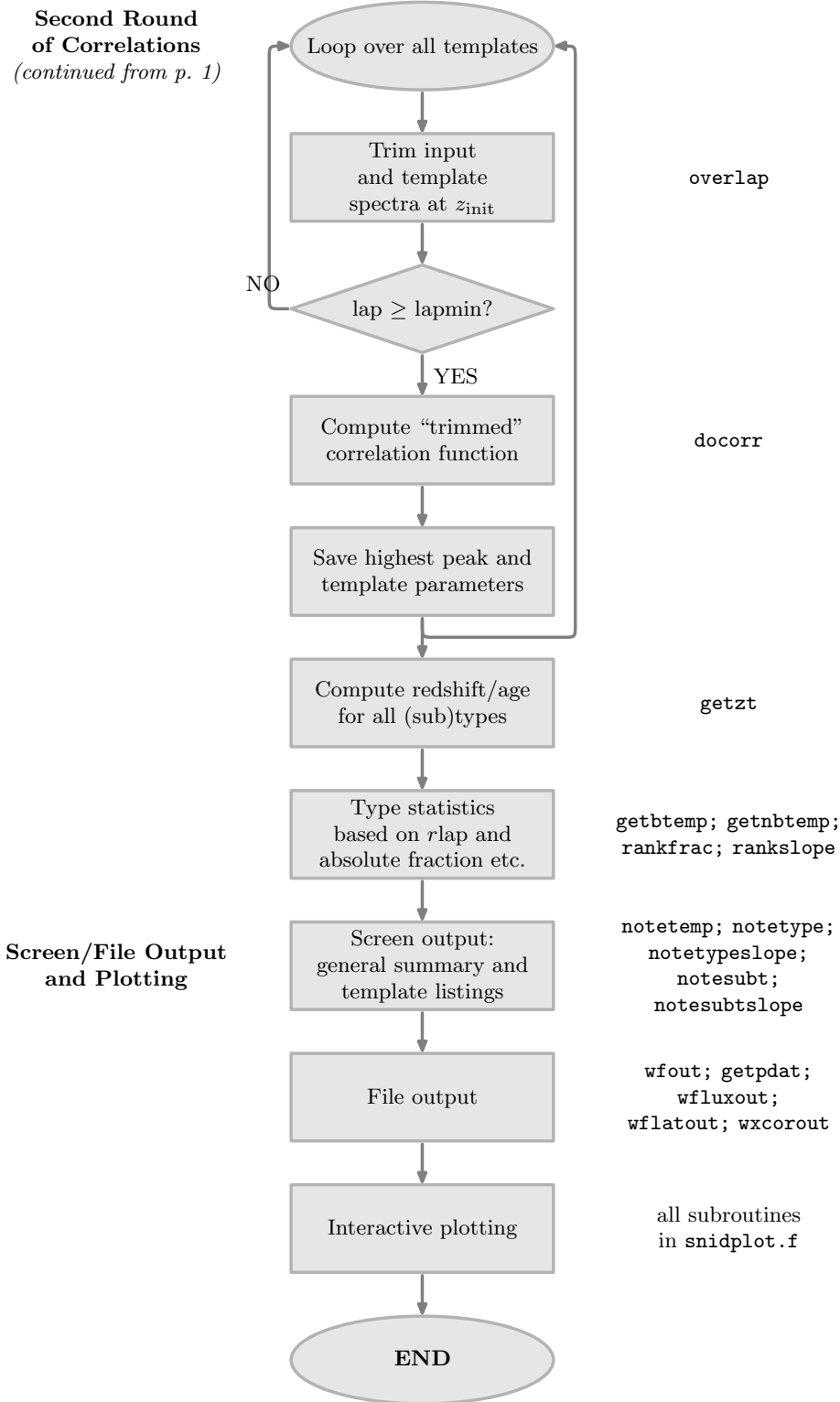
Figure 2 SNID v5.0 Flowchart ( cont. )
